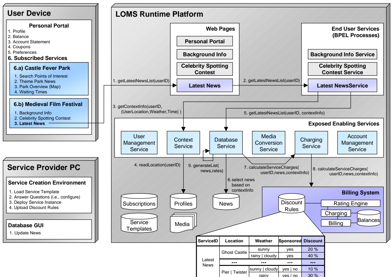
Overview of System Components and Example Message Flow of a Request for a List of Latest News
